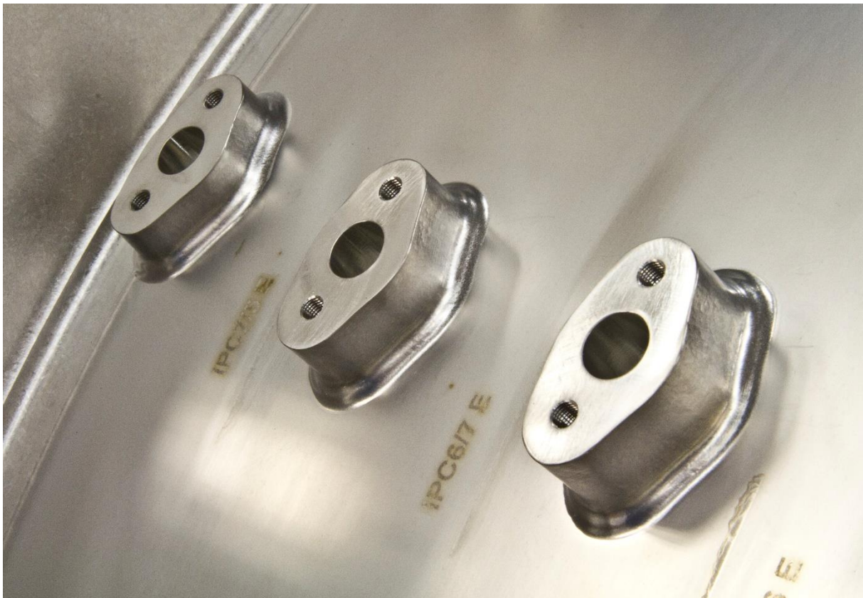
Compressor borescope bosses in Titanium, deposited by Laser Metal Deposition with wire. Picture courtesy of GKN Aerospace Engine Systems.
